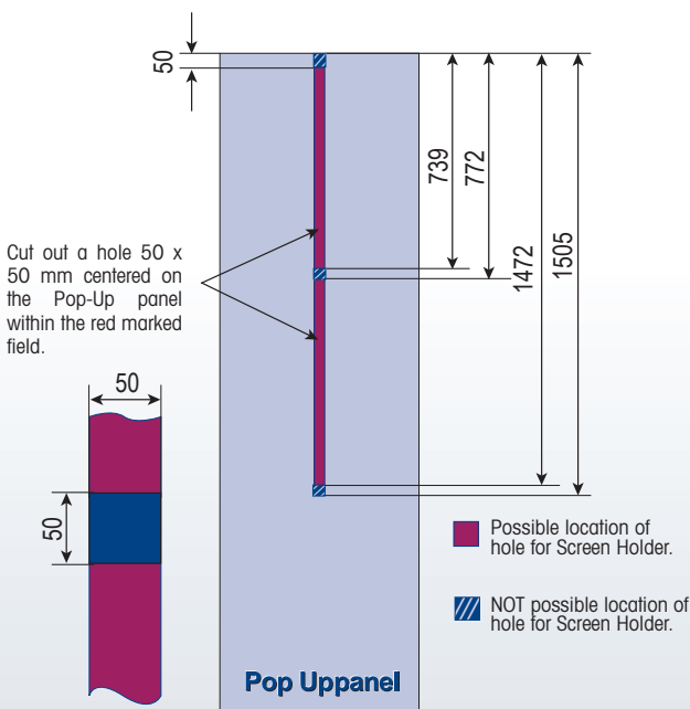
Making holes in the panel for the Screen Holder
